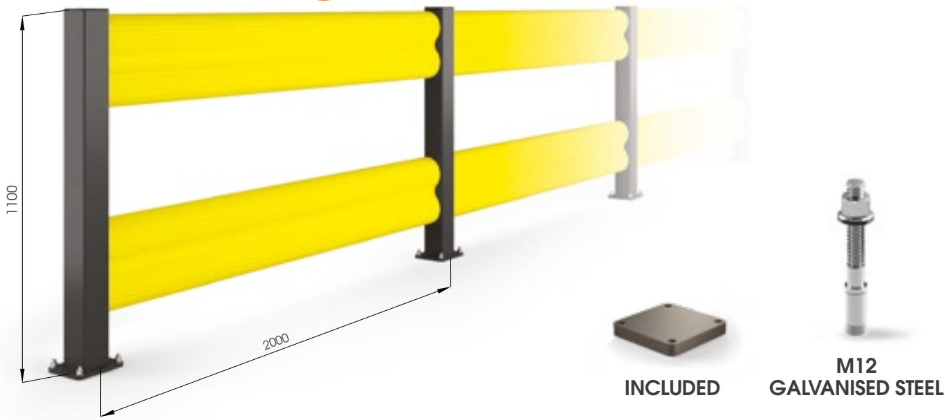
BFLEX.COM/2 2000x1100 MODULAR
