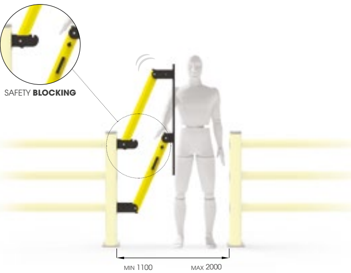
LIFT GATE 150
