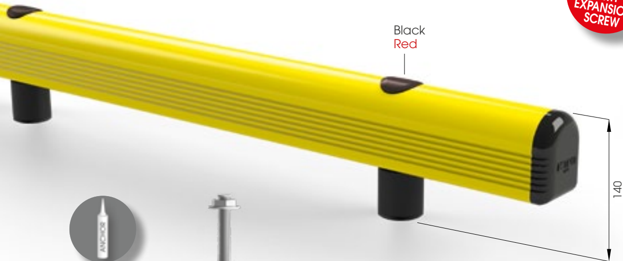
ALTERNATIVE FIXING HIGH RESISTANCE WITH RESIN M16 STAINLESS STEEL
