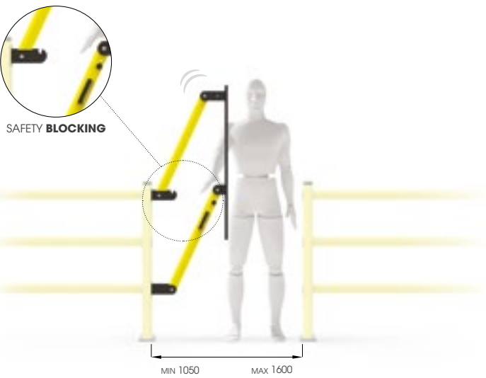
LIFT GATE 90
