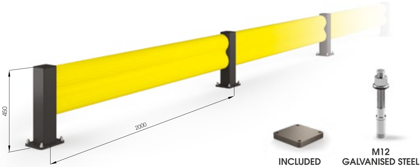
BFLEX.COM/1 2000x450 MODULAR
